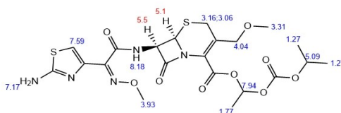
ChemNMR 1 H Estimation
